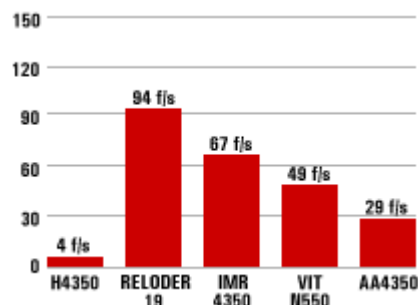
Extreme Velocity Spread For Temperatures Between 0° - 125°
