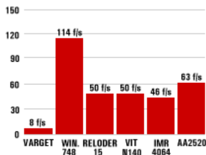
Extreme Velocity Spread For Temperatures Between 0° - 125°
